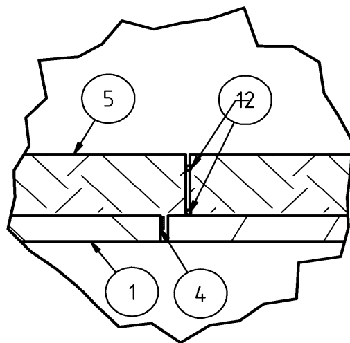
Detail E
