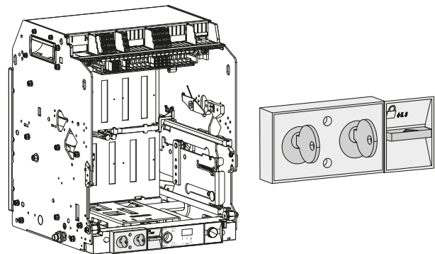
2 key locks mounted on the locking device 1 padlocking and position acknowledgement tab for HW2 and HW4 circuit breaker.
