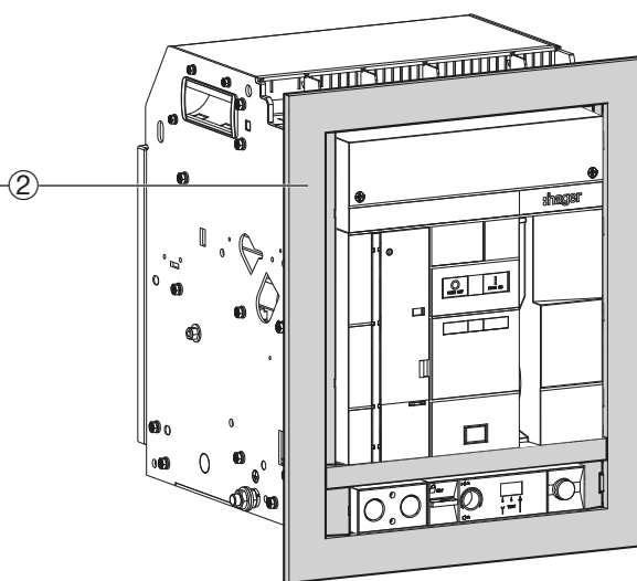
Example of an HW2 withdrawable circuit breaker
