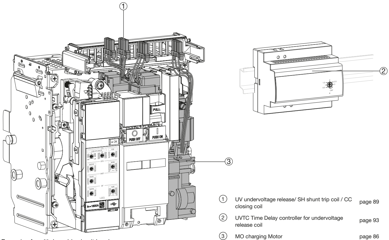
Example of a withdrawable circuit breaker
