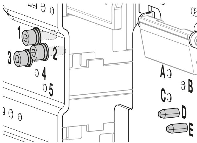
Example of installation with the combinations 123 for the chassis and DE for the HW1 circuit breaker.
