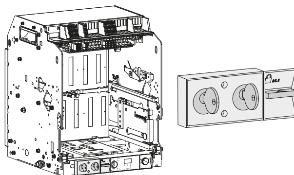
2 key locks mounted on the locking device 1 padlocking and position acknowledgement tab for HW2 and HW4 circuit breaker.
