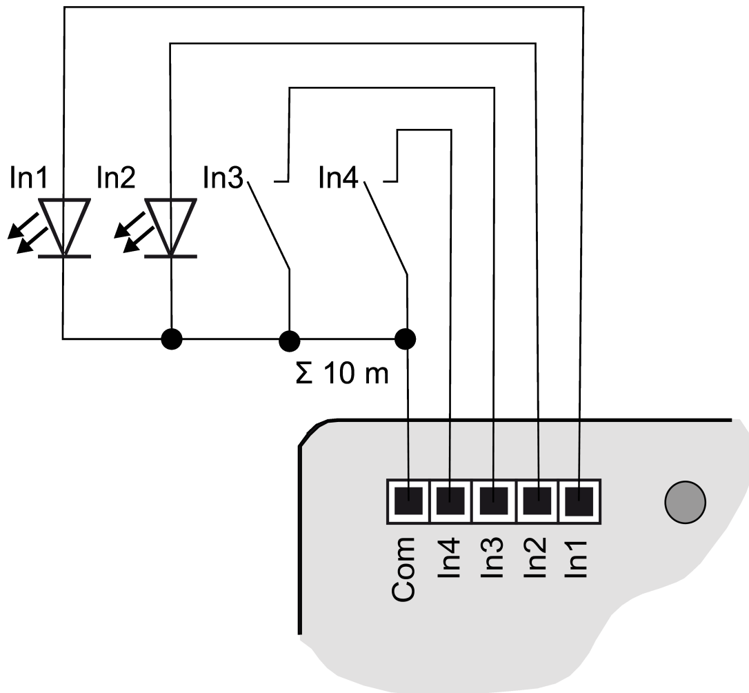
Figure 6: Connection example: push-button interface 4-gang
