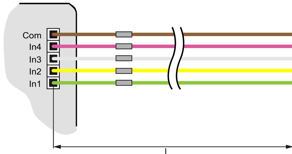
Figure 4: Maximum cable length
