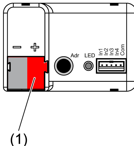
Figure 3: Bus connection
