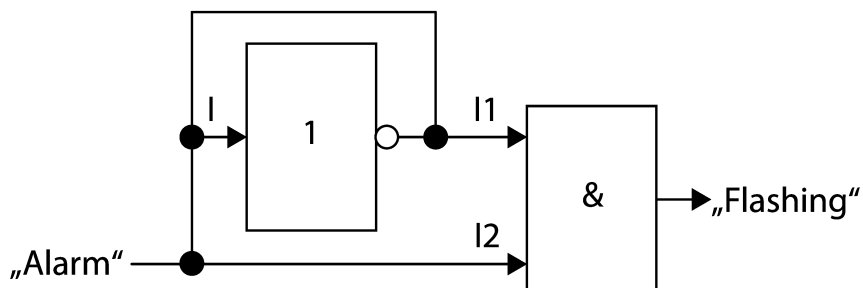
Figure 14: "Flashing" diagram
