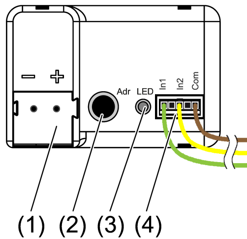
Figure 1: "2-gang" device variant
