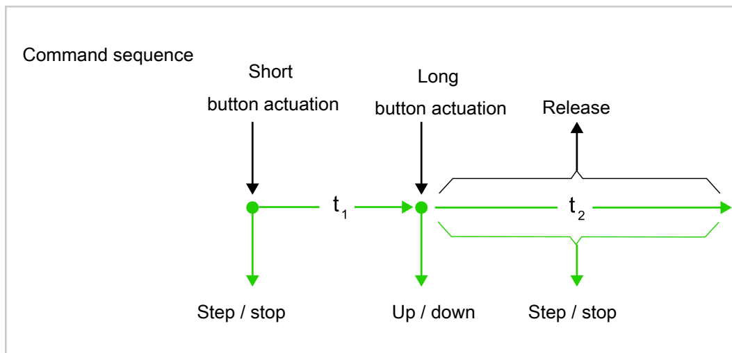
Figure 6: "Step - Up/down - Step" operating concept
