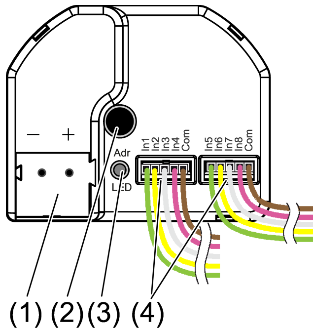
Figure 1: Front view
