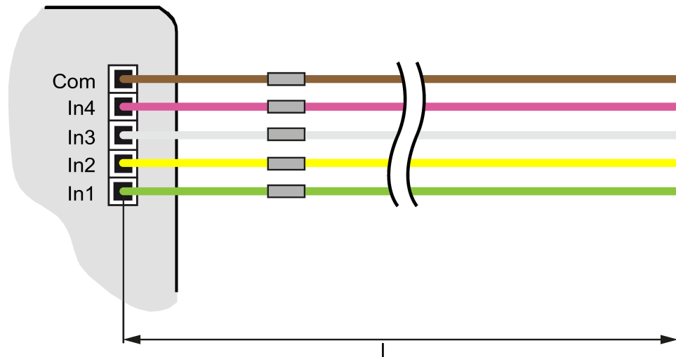
Figure 3: Maximum cable length
