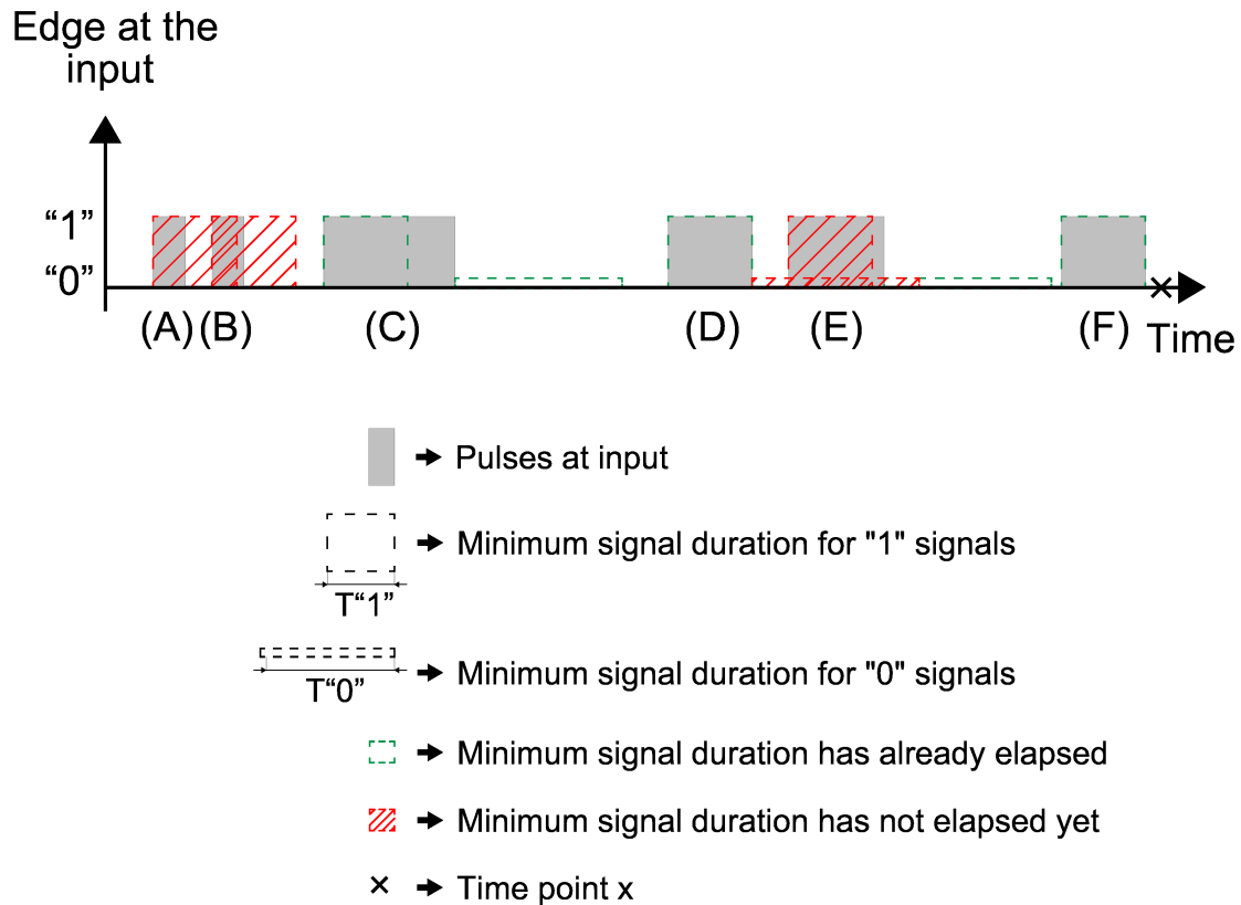
Figure 15: Example of setting the minimum signal duration
