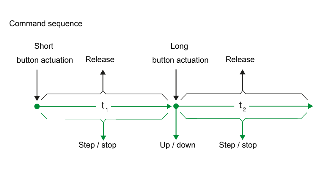
Figure 9: "Up/down – Step or step" operating concept
