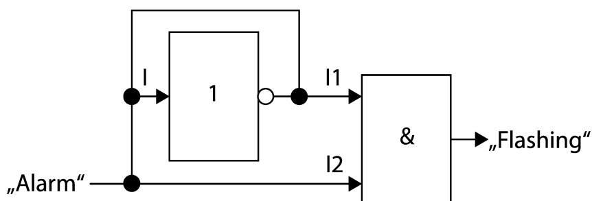
Figure 16: "Flashing" diagram
