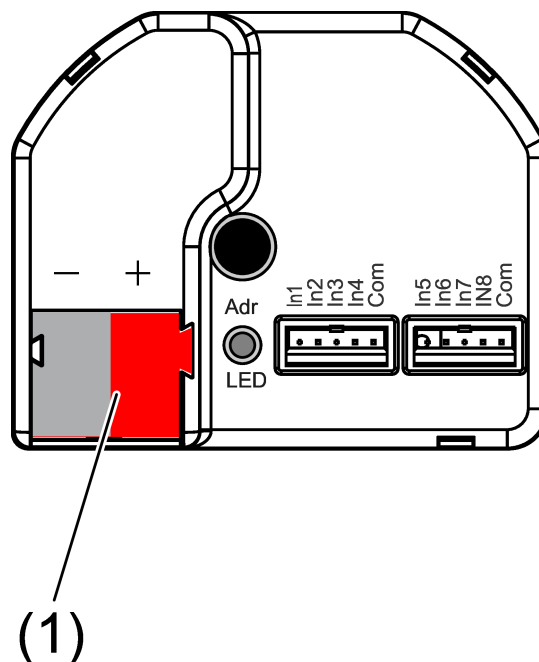
Figure 2: Bus connection
