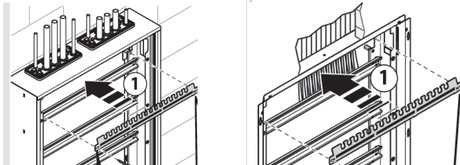
Mounting of the cable strain relief bar
