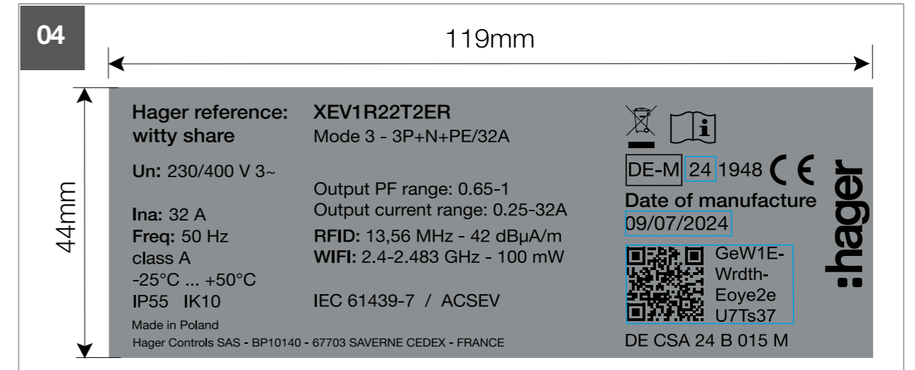
Fig 7: Typenschild
