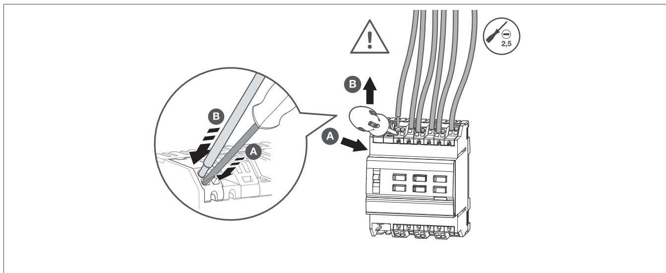
Fig. 13: Disconnecting the connection cables
