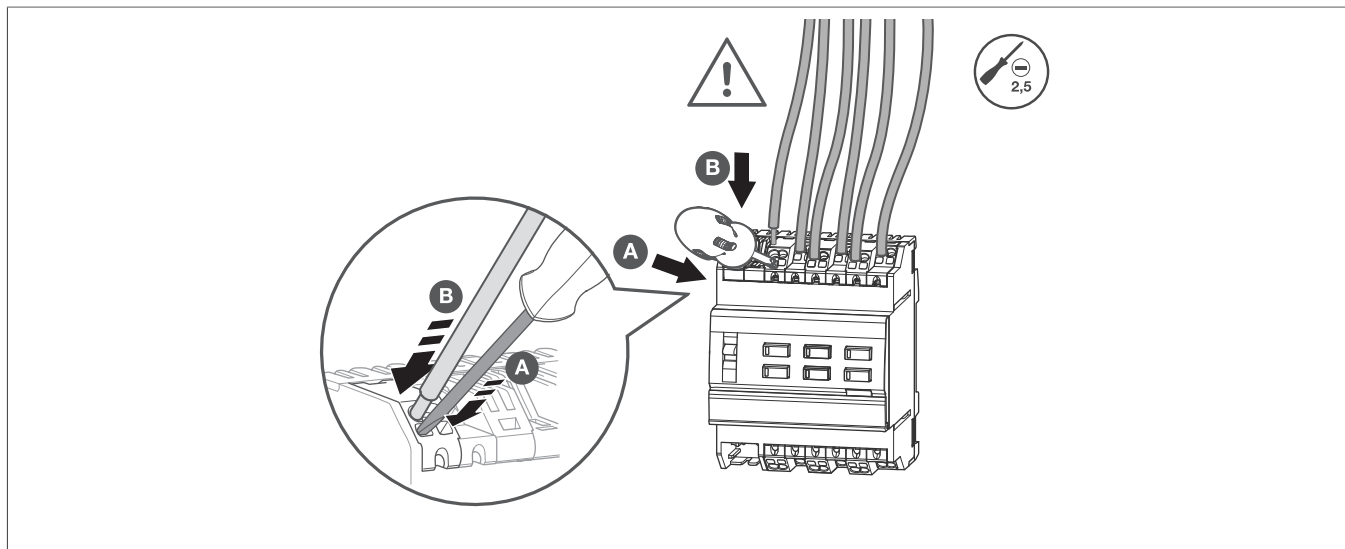
Fig. 5: Connecting the device
