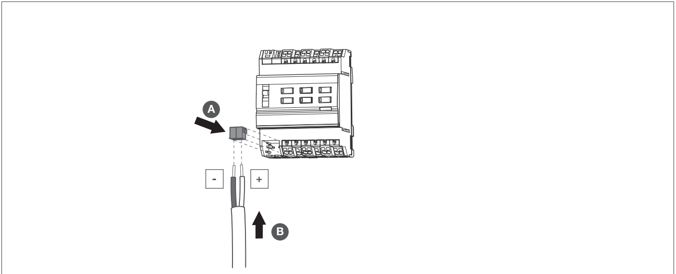
Fig. 7: Connecting the bus connection terminal
