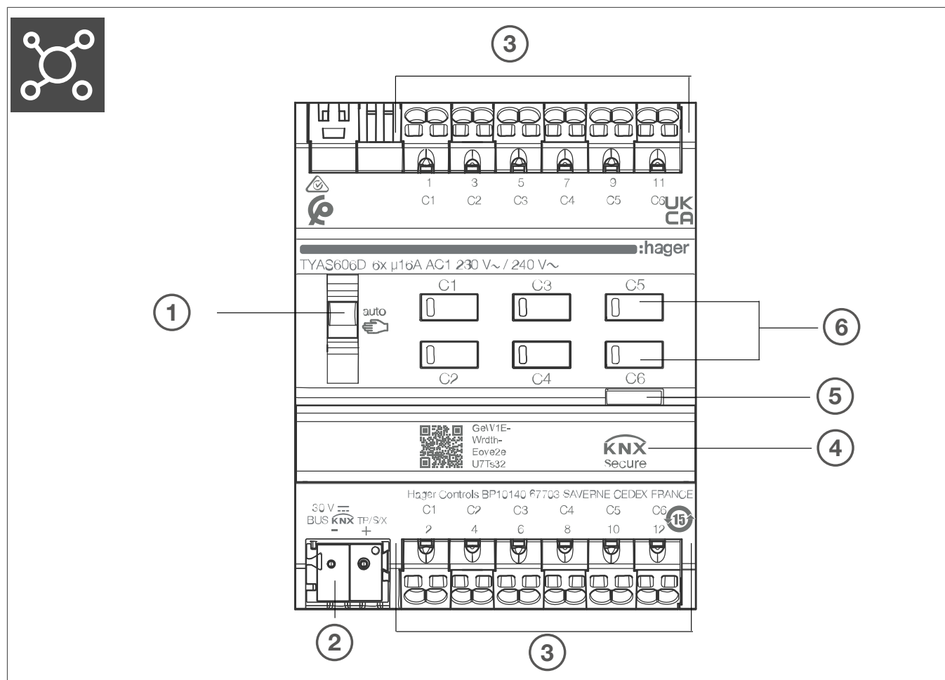
Fig. 3: Design and layout of the device
