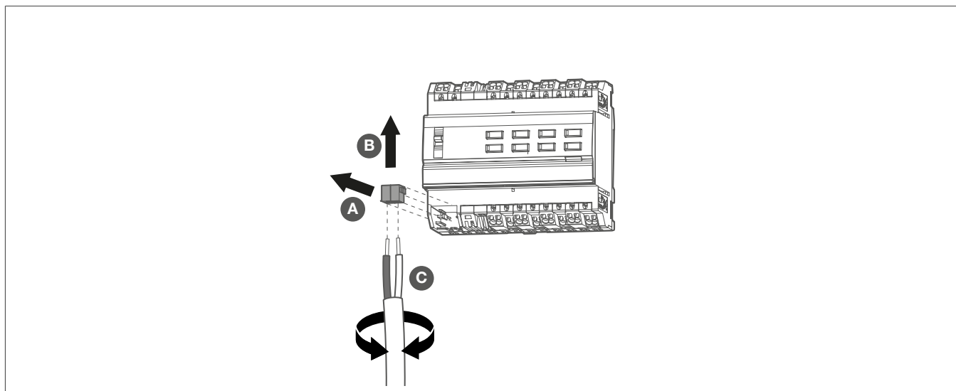
Fig. 14: Removing the bus connection terminal
