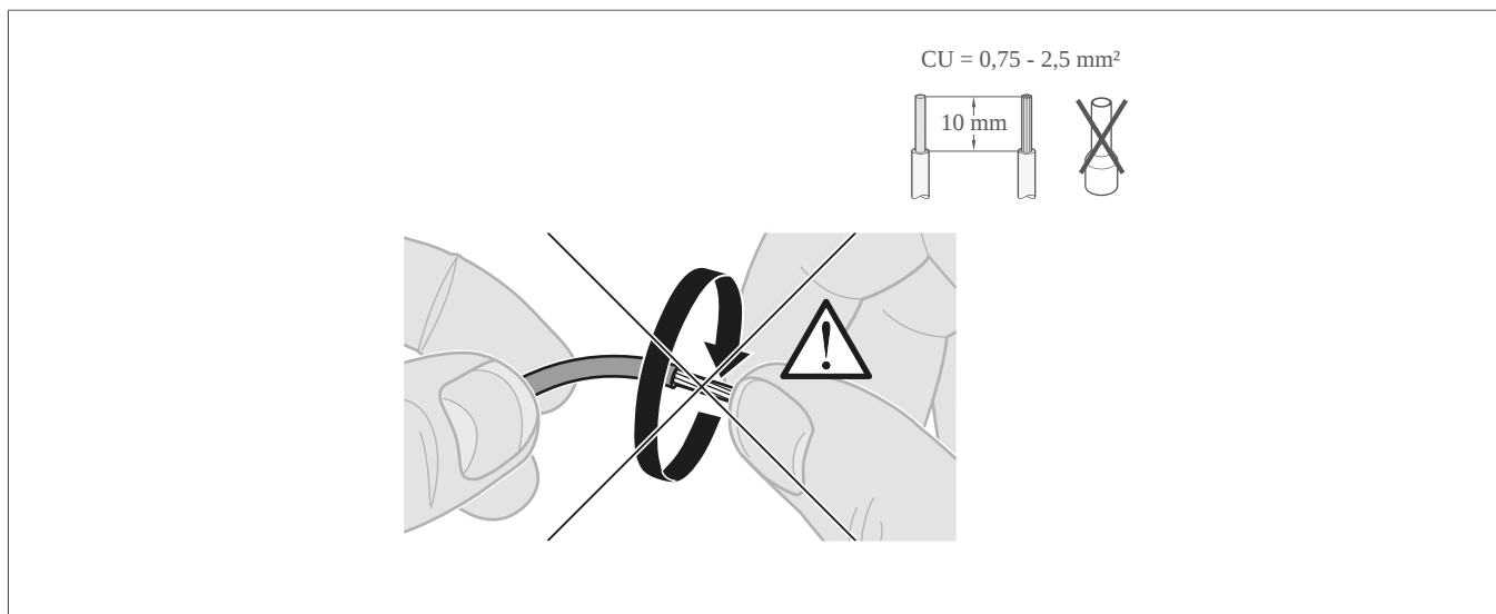
Fig. 6: Stripping length and wire cross-section
