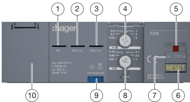
h3+ P250 combined with RCD add-on block
