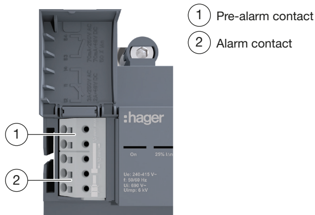
Auxiliary terminals on RCD add-on block
