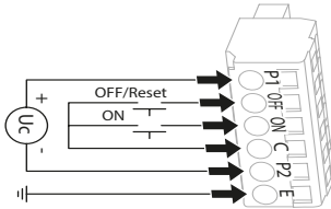
Terminal Motor operator
