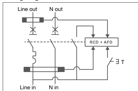
Fig 5: Wiring diagram
