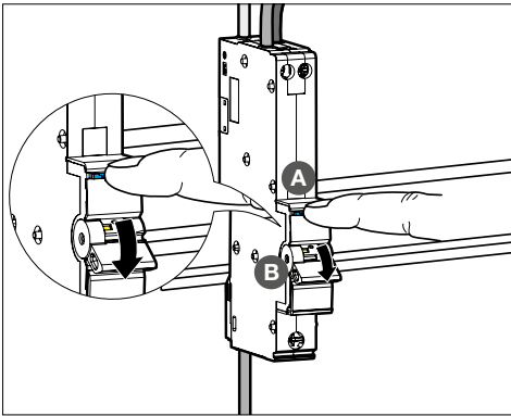
Fig 6: Testing the device ● Short press the test button T . The RCBO-AFDD tripped, i.e. the circuit must switch off.
