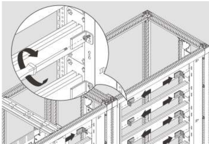
Enclosure middle
