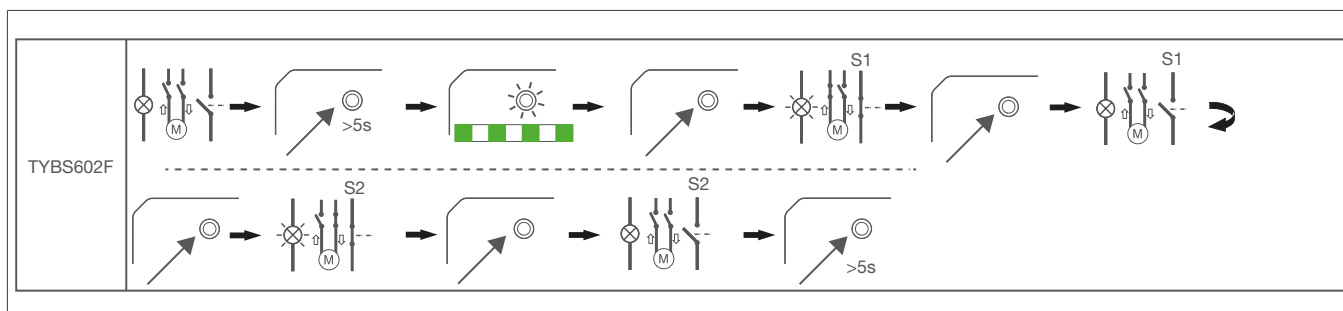
Fig. 11: Functional test
