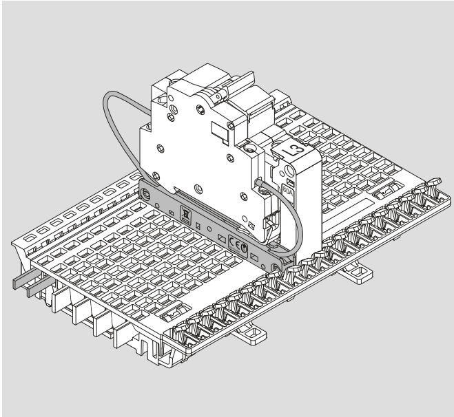
2a uniway UW-AB-xxx
