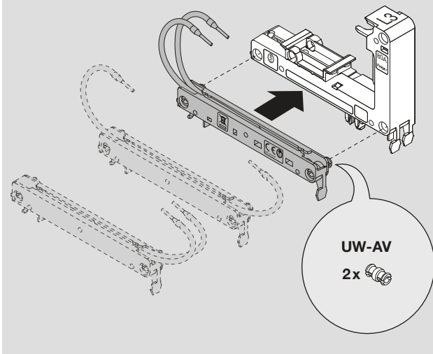
2a uniway UW-AB-xxx
