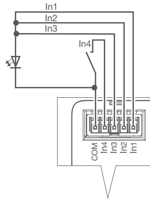
Fig. 6: Connection example for parallel-connected outputs
