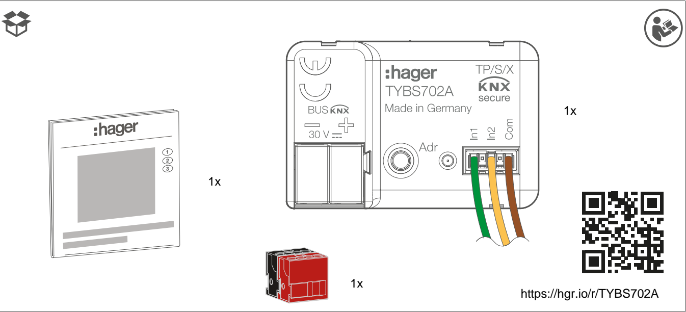
Fig. 1: Scope of delivery TYBS702A
