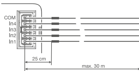
Fig. 4: Max. cable length per cable set
