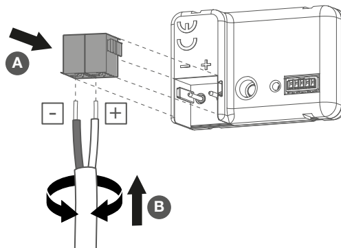
Fig. 3: Connecting the bus cable
