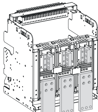
Vertical / front
