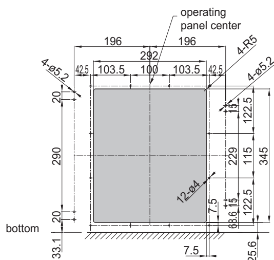
Panel door cut-out for dust cover (mm)
