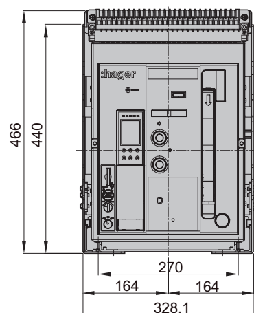
Front view (mm)
