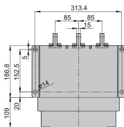
Vertical terminal connection (mm)
