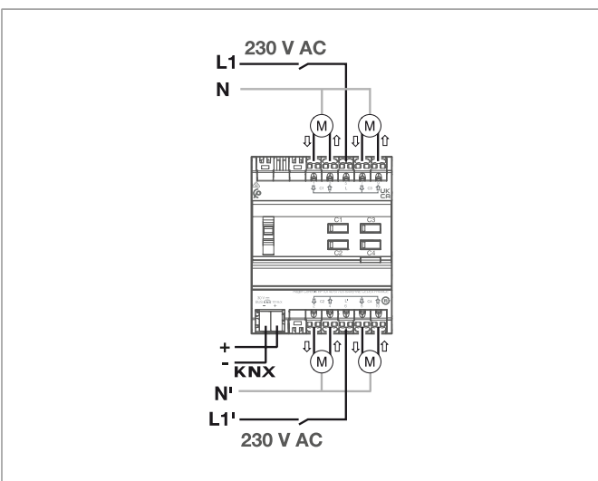
Fig. 5: Connecting the device
