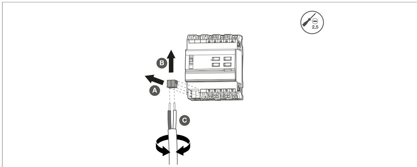
Fig. 13: Disconnect the KNX bus connection terminal
