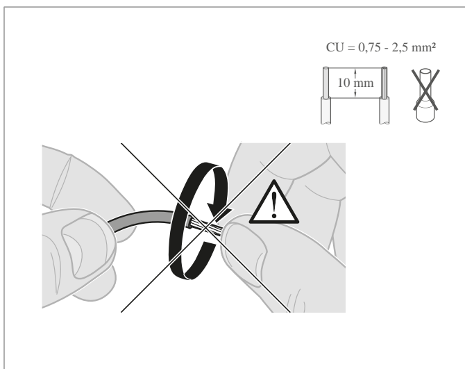
Fig. 4: Prepare connection cables.
