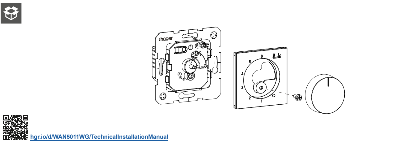
Fig. 1: Scope of delivery WAN5011xx
