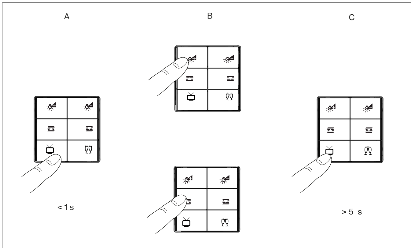
Fig. 15: Scene call-up
