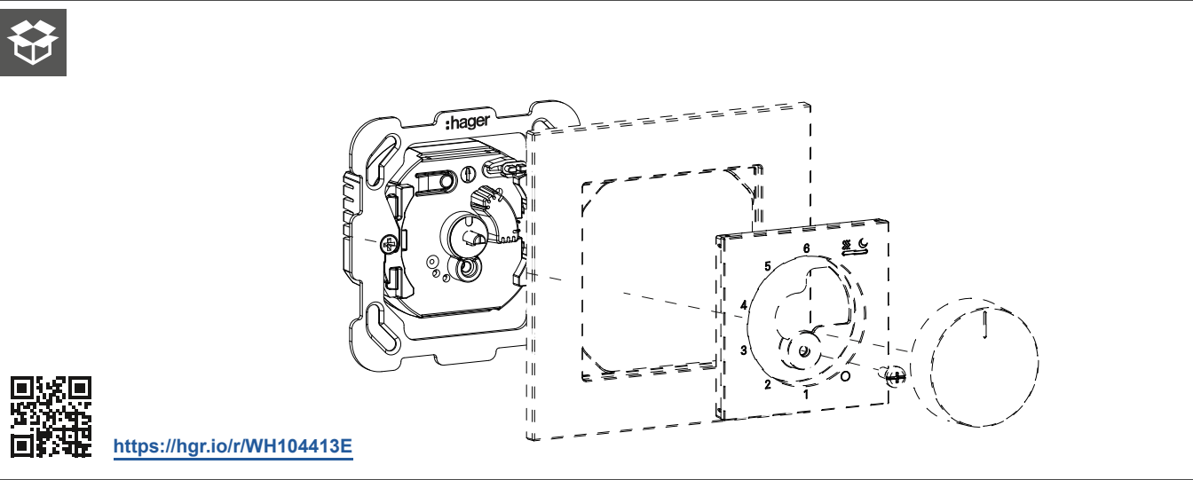
Fig. 1: Scope of delivery of the electronic room temperature controller 230 V/15 W
