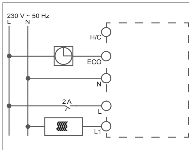
Fig. 6: Electrical connection for heating
