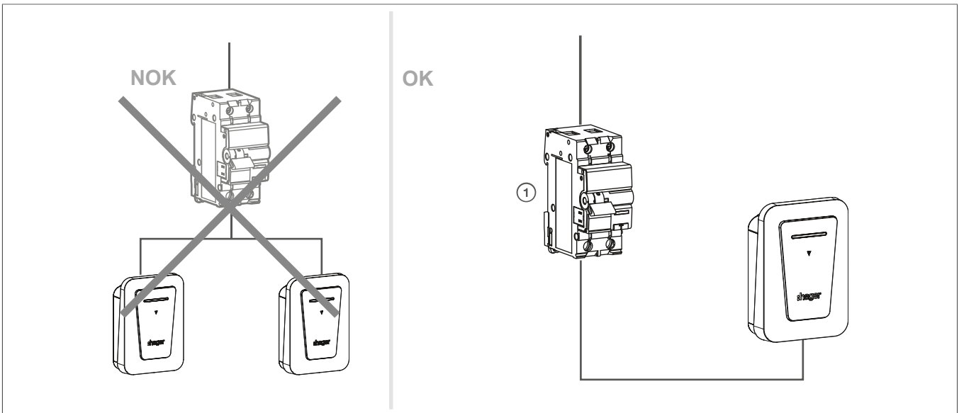
① 1P+N 6kA C-40A 30mA A Class
