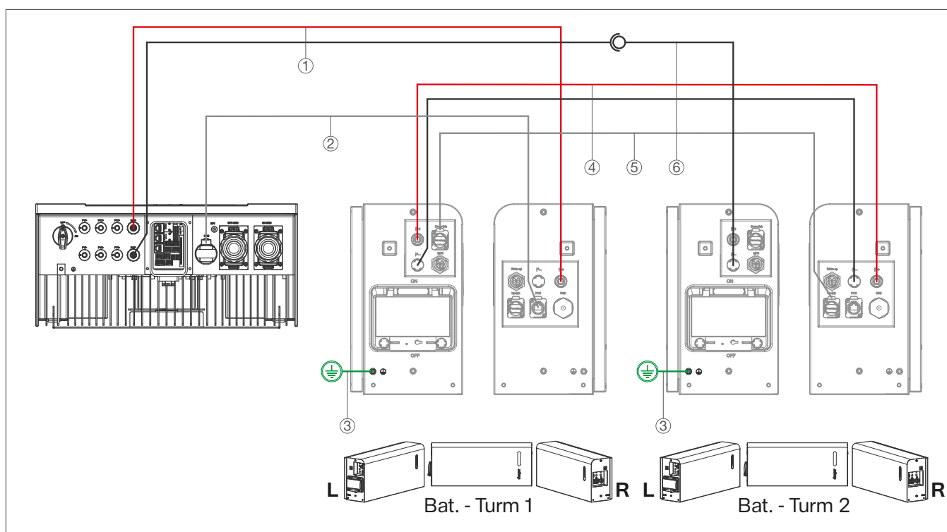
Fig. 30: Retrofitting of battery modules
