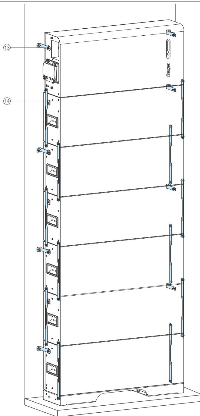
Fig. 22: Overview of all fasteners (see image)
