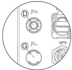
BMS Left Side (stackable Battery System 1)
