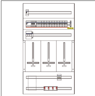
ZW313F-S-004_AUFBAUPLAN_PD
