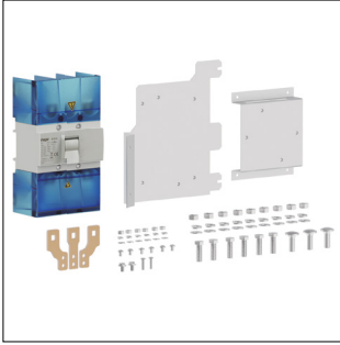
Hager JPA0S160 blue modular electrical switch disconnect and mounting kit
