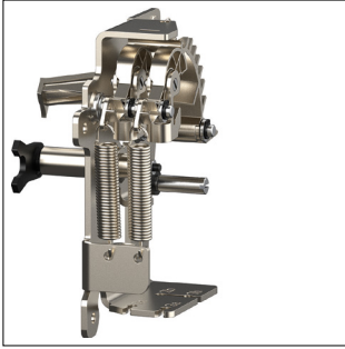
Plate for mechanical interlock HW1 DO Coupling (Type 3C) - 1 Plate/ACB (MI)
