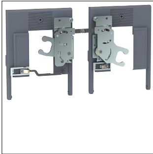
Link interlock kit x630/P630 - 3P
