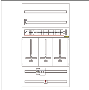
ZW313F-B-004_AUFBAUPLAN_PD
