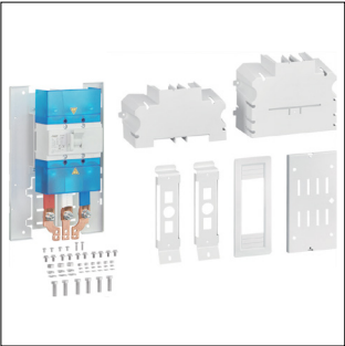
main incomer 250A switch link kit
