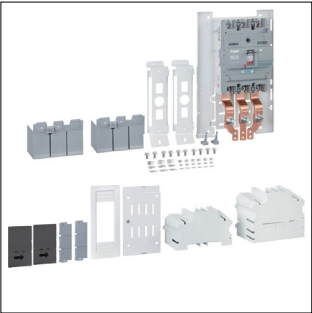
main incomer 200A MCCB (X250) link kit
